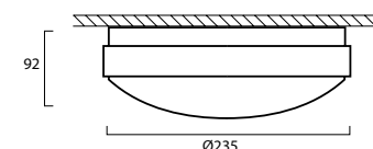
Giotto LED G2 235 Surface
