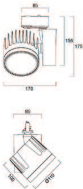
Dimensions (mm)
