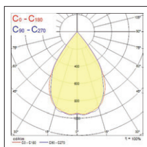
Raxa 600 UGR19 3000K
