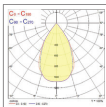
Raxa UGR19 1500 3000K
