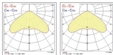
SportsBay 12800lm
