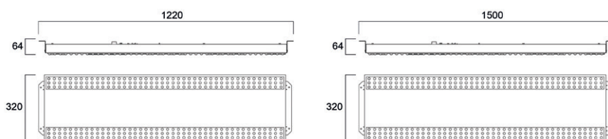
SportsBay 1200
