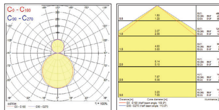
Opaal direct/indirect
