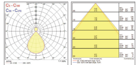
Reflector direct/indirect
