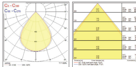
Reflector direct
