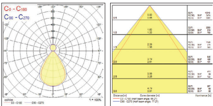
Prismatisch direct/indirect
