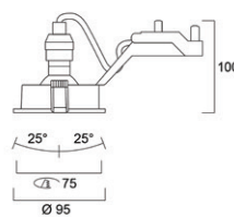
Inset Trend / Instar Trend SW IP44
